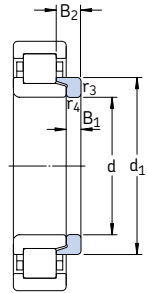
Aro angular
